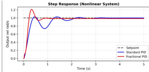
Figure 3. Step response.
